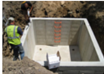
Underground Storage
